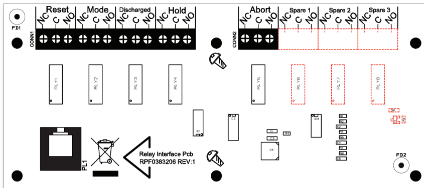
Figure 1 - Output Expansion Relay Board PCB Layout
